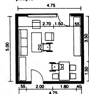
⑥ Living/dining room (4-5 people: 23.75m 2 )
